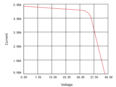
Module IV Graph 150W
