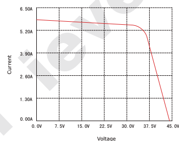
Module IV Graph 180W
